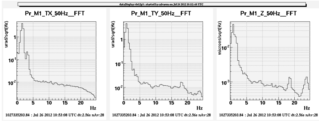
Figure 10: The spectrum of excitations on M1 when it is free E.G. not being controlled and no injected excitation.
