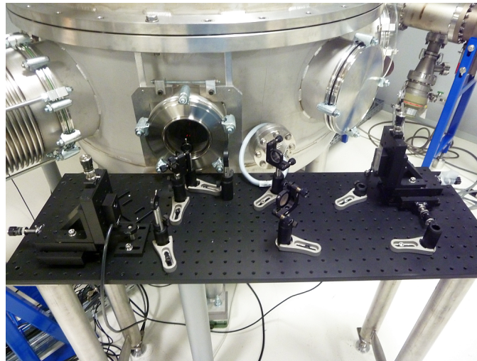
Figure 8: Local Control photodiode assembly from M2.
