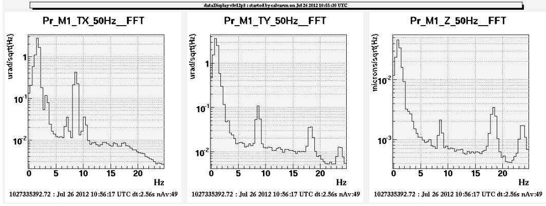
Figure 11: M1 spectrum after injecting an 8.6\text{Hz} signal on \theta_x . Note the relatively large concomitant excitation in \theta_y
