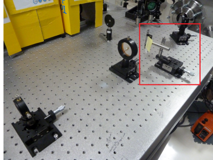
Figure 16: Typical setup used for razor blade measurement
